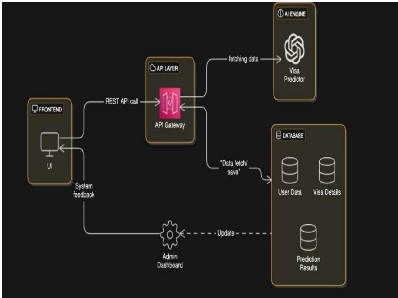
Figure 2.2.11: Component diagram
