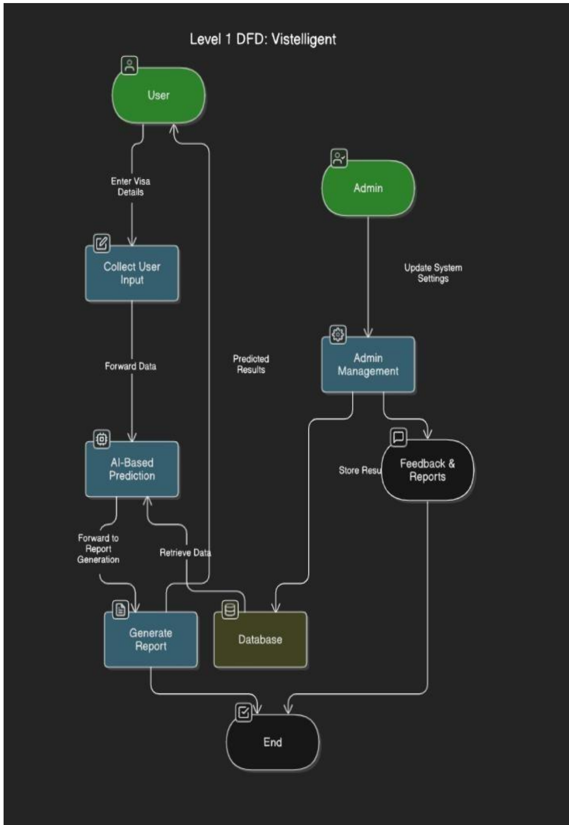
Figure 2.2.10: DFD
