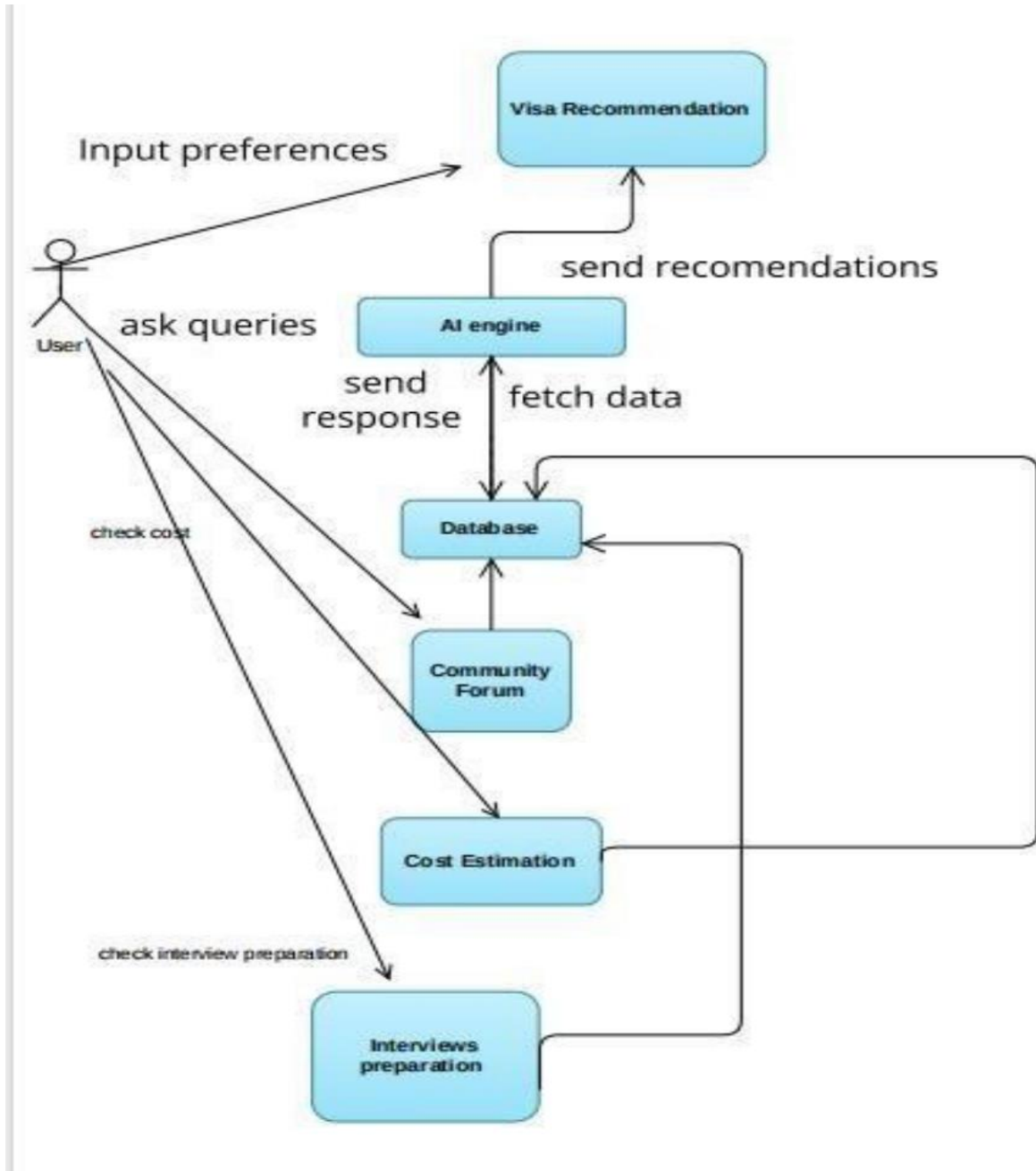
Figure 2.2.3: Collaboration diagram
