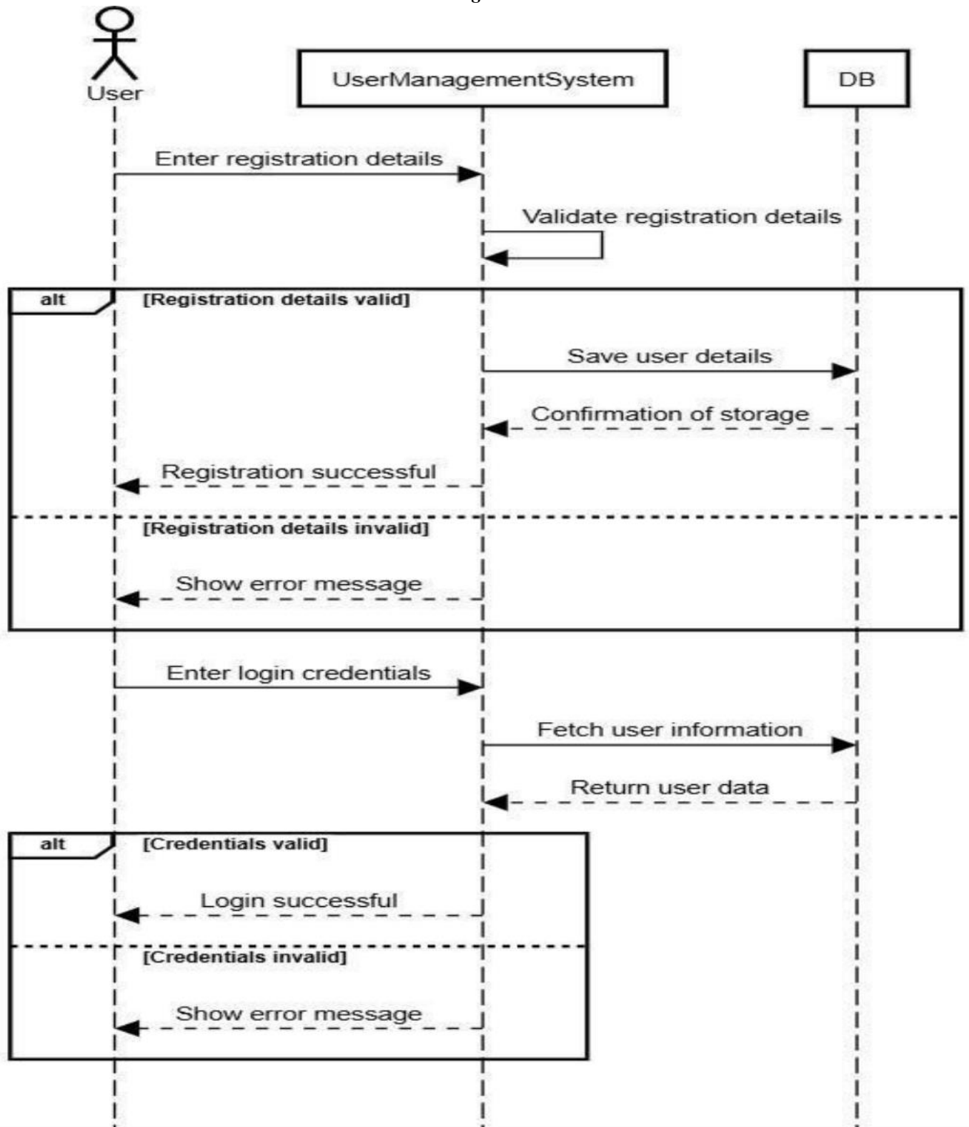
Figure 2.2.6: User Management
