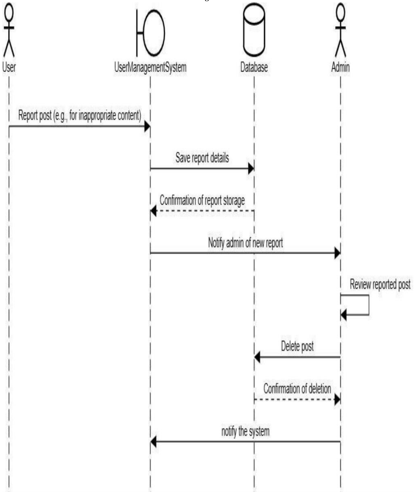
Figure 2.2.8: Report post
