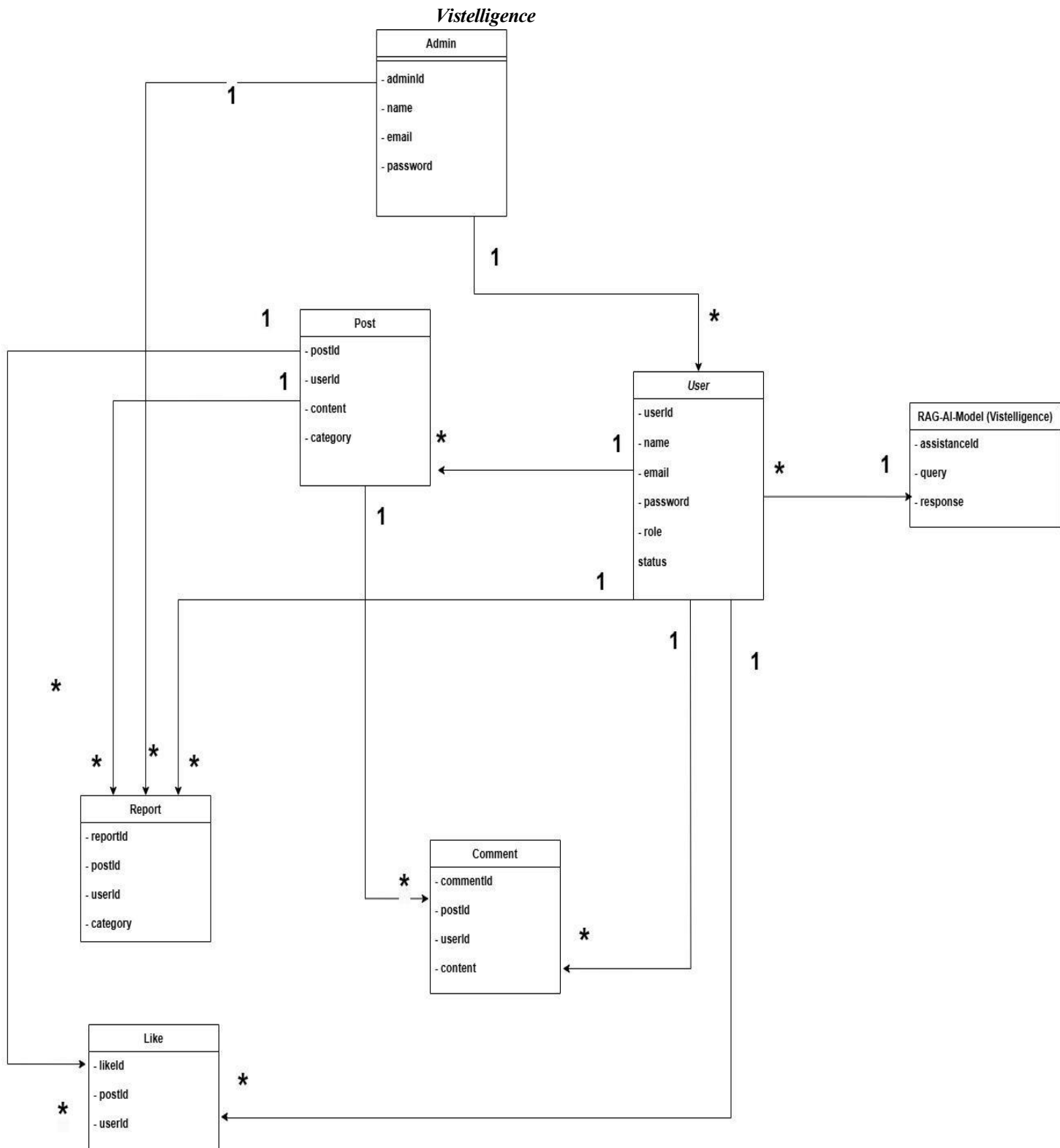
Figure 2.1.1: ERD diagram:
