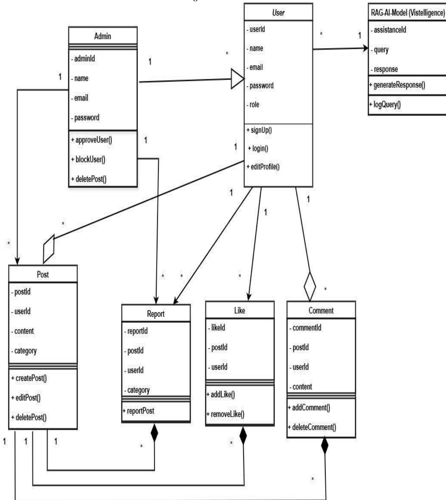
Figure 2.1.2: Class diagram
