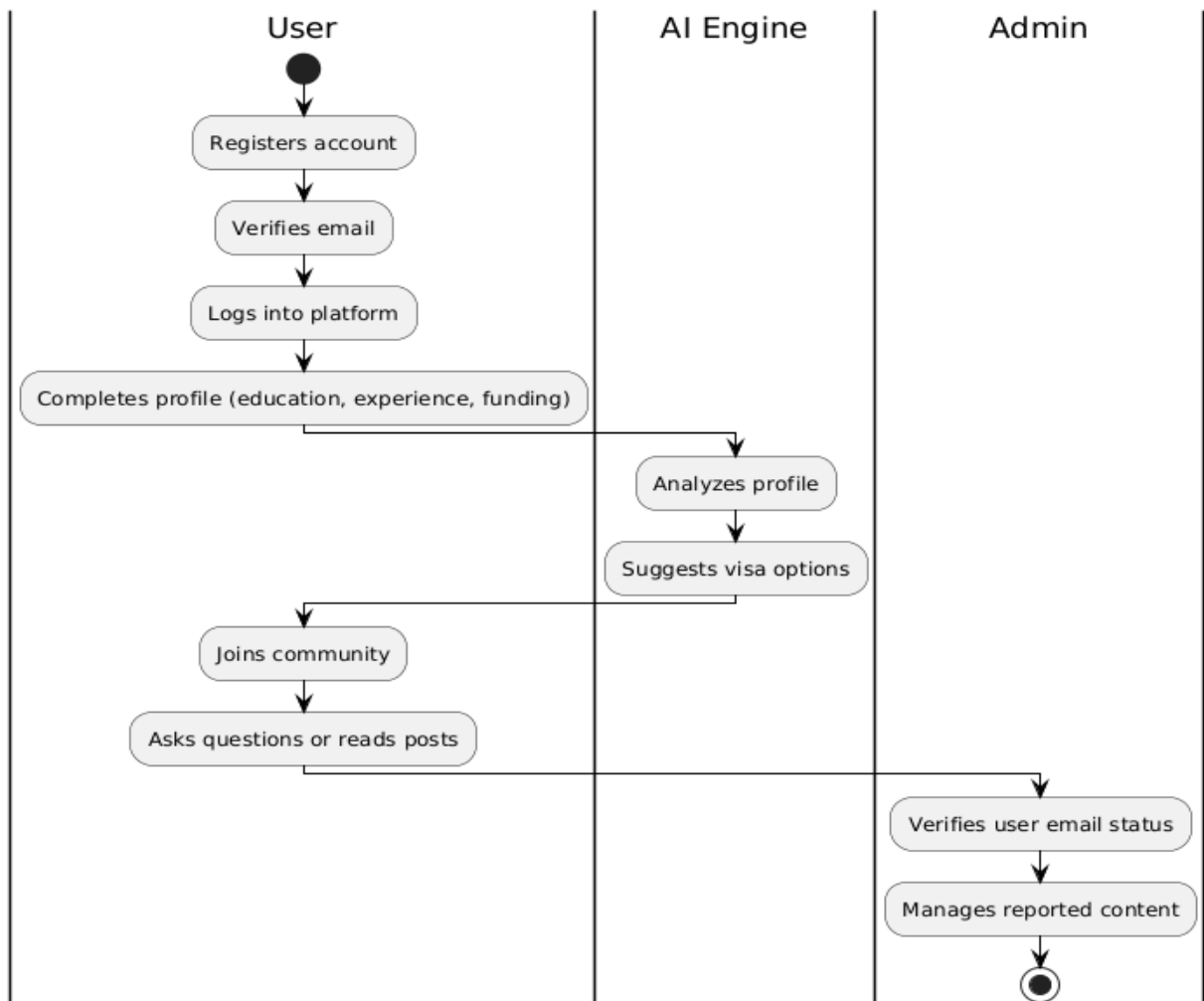
Figure 4.1: Swimlane daigram
